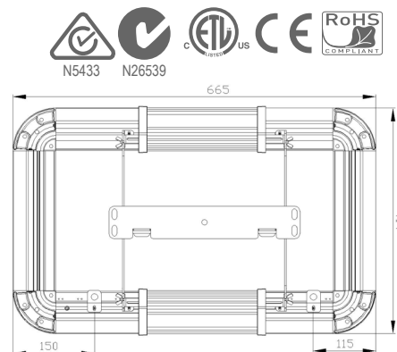
Schematic of 150W Floodlight
