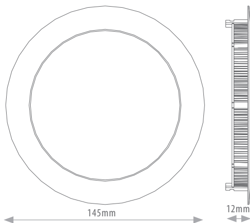
SCHEMATIC OF CORONA-145C-8W
